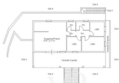
PIANO TERRA
