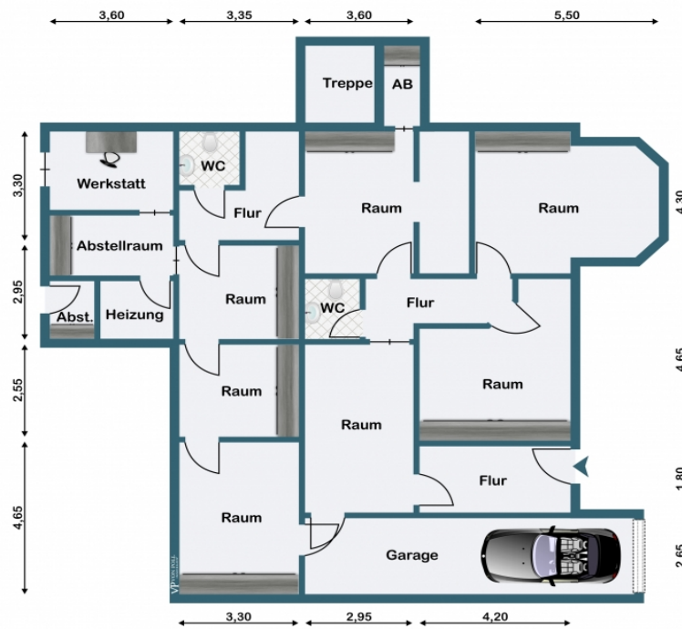
33_Souterrain
