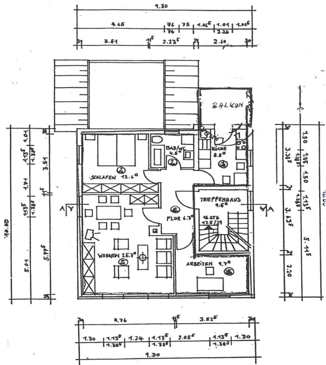
GRUNDRISS 1.0G M 1:100
